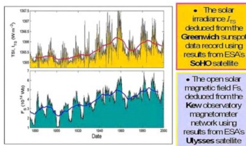
Figure 23: Reconstruction of the solar irradiance and the open magnetic flux from 1880. After (13).
