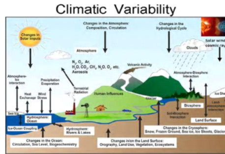
Figure 5: The complexity of the climatic variability. The author added in the up right corner the solar wind and cosmic rays as a possible source of climate forcing; the latter one is poorly mentioned in most of the reports, because still controversial; sensitivity of the ozone density in the tropopause could be also a radiative forcing.
