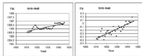
Figure 15: An example of the irradiance (TSI) trend, left, and Earth's temperature trend, right, during the years 1910-1945. After (20).
