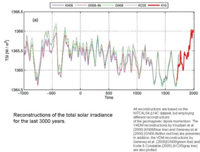
Figure 24: Reconstruction of the total solar irradiance for the last 3000 years. After (27).
