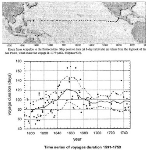
Figure 28: From the ship log-books, time travels can be reconstructed. This figure shows the duration of a travels from Acapulco to Manila between 1591 and 1750. It can be seen that the winds were blowing lower during the deep solar Maunder Minimum.
